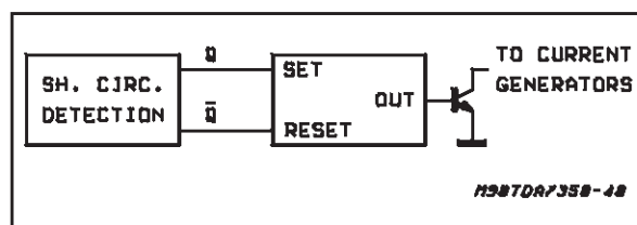
Figure 39: Restart Circuit
