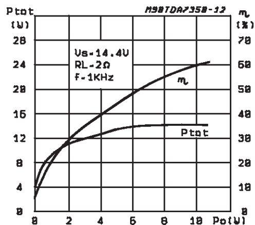
Figure 19: Power Dissipation &amp; Efficiency vs. Output Power (Stereo)
