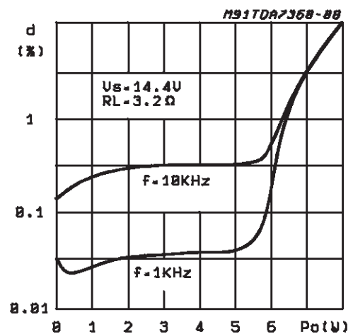
Figure 12: Distortion vs Output Power (Stereo)
