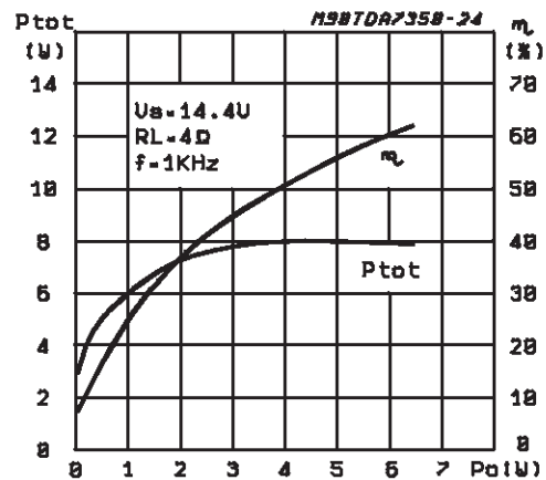
Figure 20: Power Dissipation &amp; Efficiency vs. Output Power (Stereo)
